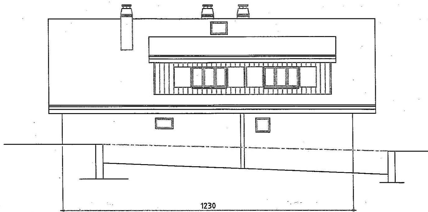
FACADE NORD—OUEST
